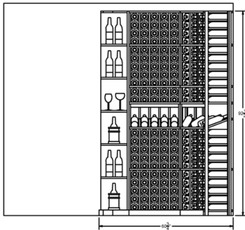
ELEVATION -A-
